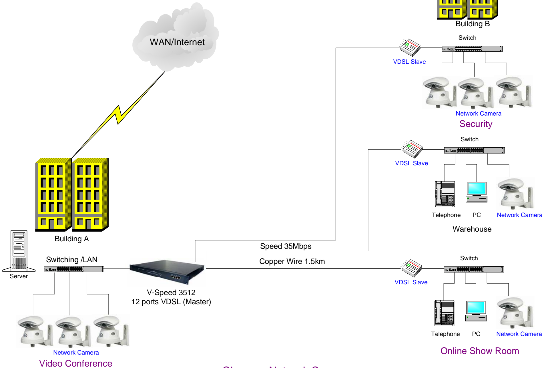
Observer Network Camera with Multiport VDSL Solution
